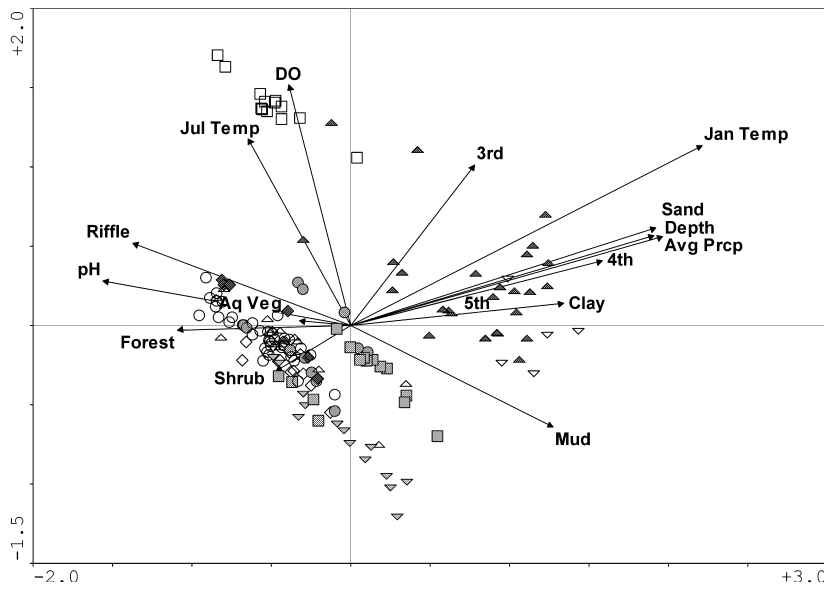
Figure 4 Sample score ordination on canonical correspondence analysis (CCA) axes 1 and 2 (axes x and y, respectively) from CCA of the taxonomic data set, with significant local- and regional-scale environmental variables (Table 3). Brazos (▲), Devils (□), Frio (○), Hondo (◆), Medina (⊙), Middle Concho (■), Concho (▣), Sabinal (△), South Concho (◇), Spring (▼), Village (▽).
